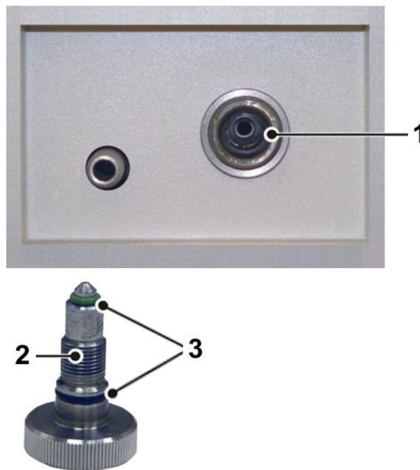
Fig. 56: Valve opening and valve core with O-rings (example, varies depending of the type of freeze-dryer)
